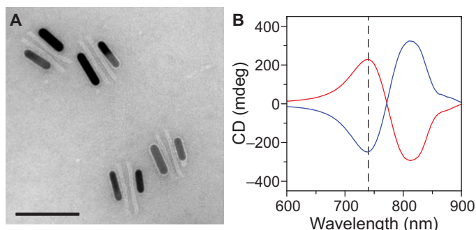
Fig. 2. DNA assembly of the plasmonic metamolecules and their chiroptical response. (A) TEM image of the plasmonic nanostructures. The structures tend to lie flat on the TEM grid. Scale bar, 100 nm. (B) Measured CD spectra of the metamolecules in the LH (red line) and the RH (blue line) state from the LH 50% and RH 50% samples at pH 5.5, respectively.
